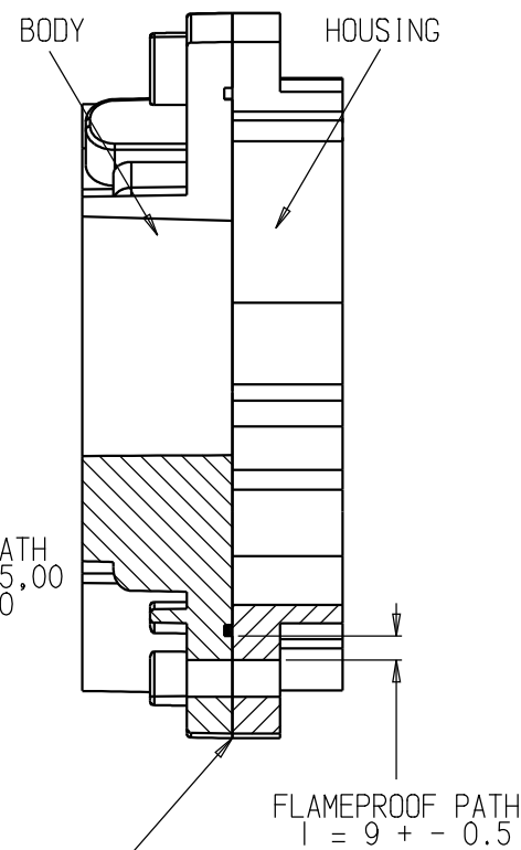
SECTION B-B
