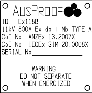
LABEL B PRODUCT LABEL FOR INSULATED END COVER
